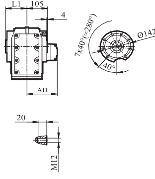
GKA/GKH/GK77
