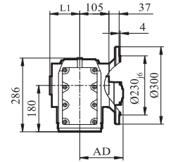
GKAF/GKHF/GKV77
