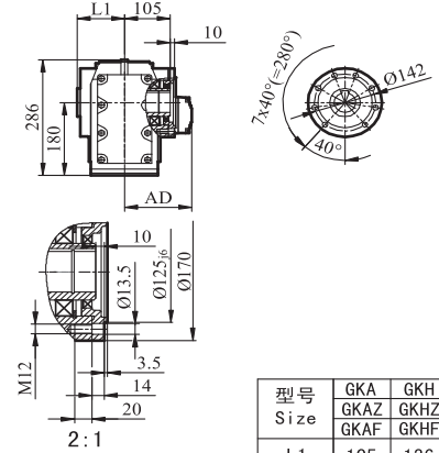
GKAF/GKHF/GKV77
