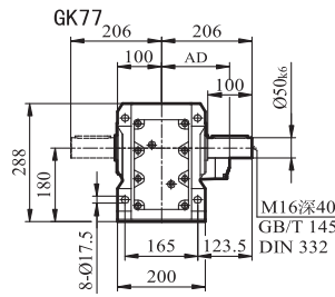
GKA/GKH/GK77
