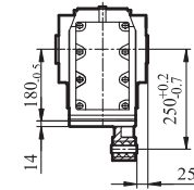
GKH/GKHZ/GKHF77输出轴
