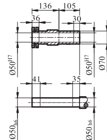
GKH/GKHZ/GKHF77输出轴
