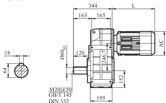
GFA/GFH/GFV87
