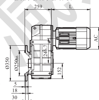
GFAF/GFHF/GFVF87
